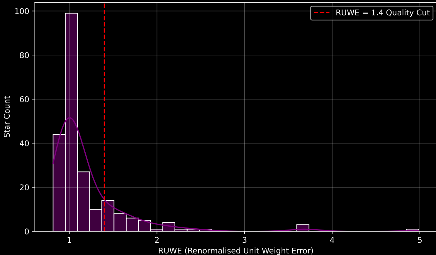
GALAH DR4 Field [8489] RUWE Distribution (n= 225)
