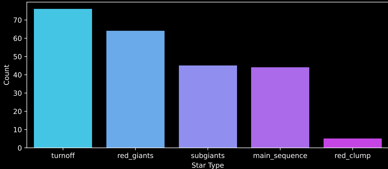
GALAH DR4 Field: [8489] Count plot of Star Type
