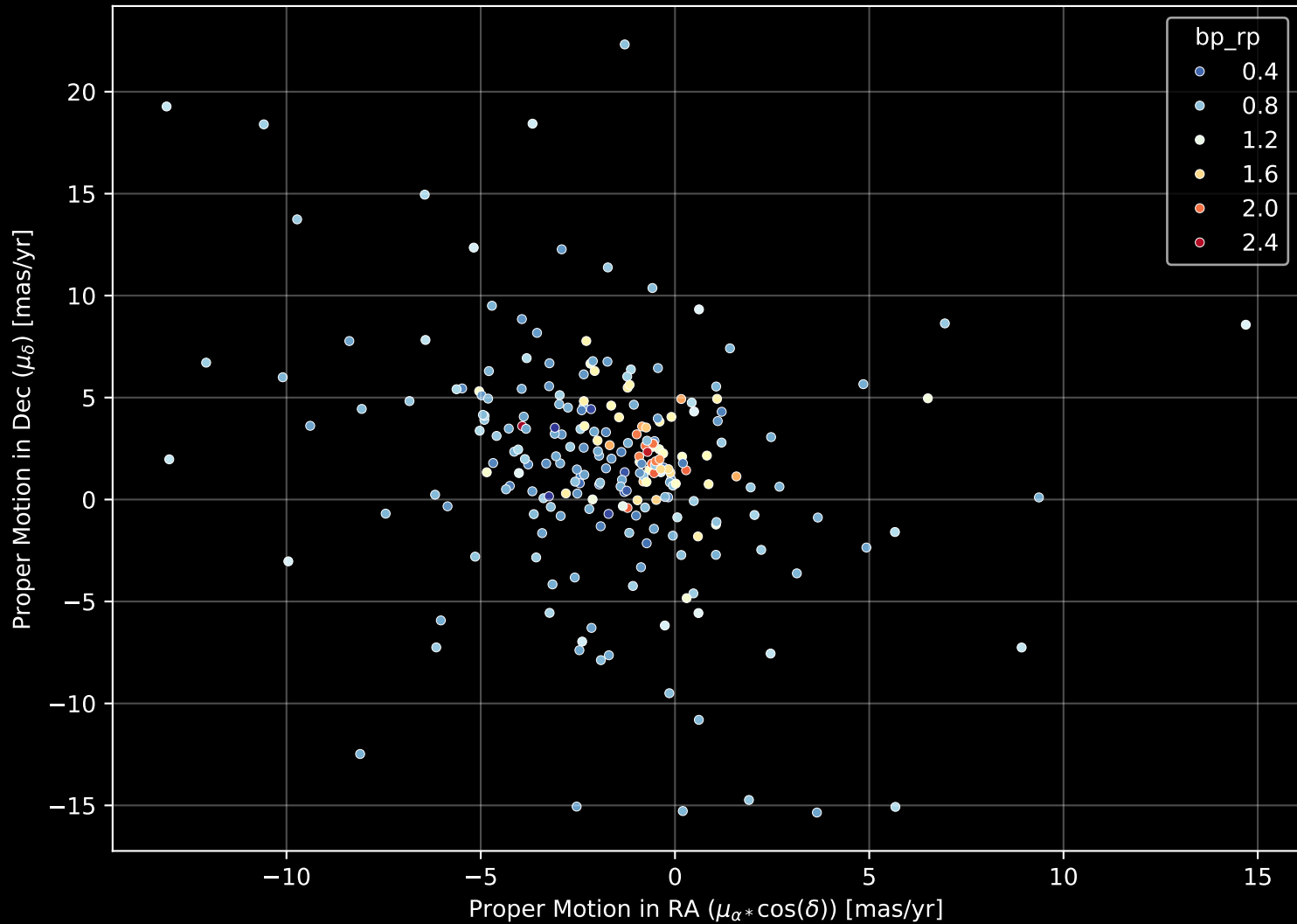
GALAH DR4 Field: [8489] Proper Motion Diagram (n= 234)
